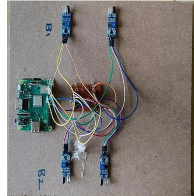
Fig 4: Without power supply
