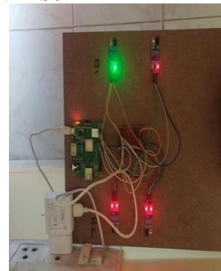
Fig 5: With power supply
