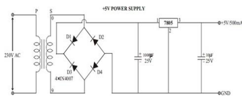
Fig .3 Circuit diagram of power supply
